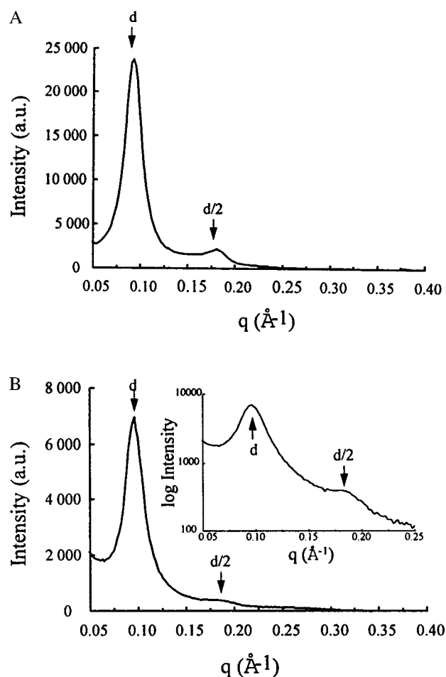
FIG. 3. SAXS scans of BGTC/DOPE-DNA lipoplexes from zone C (A) and of BGTC-DNA lipoplexes from zone C (B); in the Inset, the log of the scattering intensity is plotted as a function of the momentum transfer q . d and d/2 correspond to the first reflection and the second order reflection, respectively.
